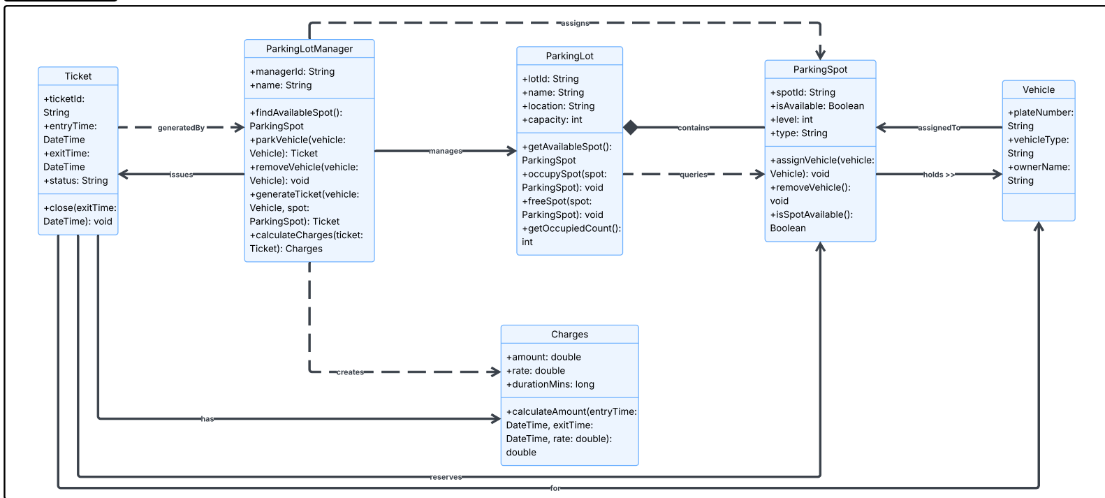
Parking Lot UML Class Diagram
